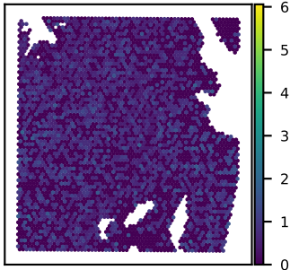
SNU51A STAG1 expression Moran's I = 0.03
