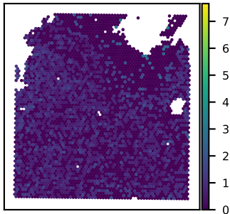
SNU21B C11orf49 expression Moran's I = 0.08
