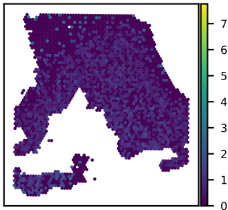
SNU18A C2orf74 expression Moran's I = 0.09
