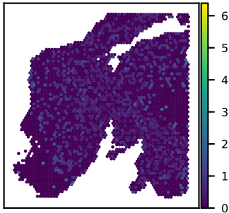
SNU24A GTPBP3 expression Moran's I = 0.02
