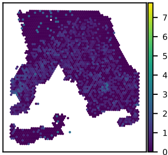
SNU18A ISLR expression Moran's I = 0.16
