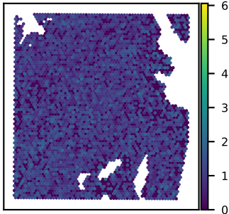
SNU51A CAMTA1 expression Moran's I = 0.01
