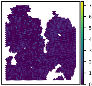
SNU27B HIST1H3A expression Moran's I = 0.05
