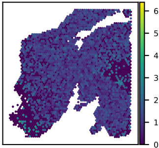
SNU24A SPEG expression Moran's I = 0.10
