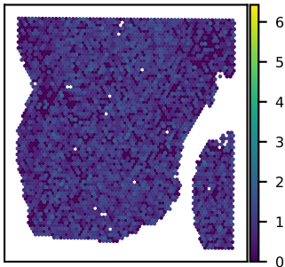
SNU25B SRGAP3 expression Moran's I = 0.05
