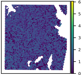
SNU51A DHX15 expression Moran's I = 0.03
