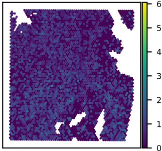
SNU51A PLXDC1 expression Moran's I = 0.10
