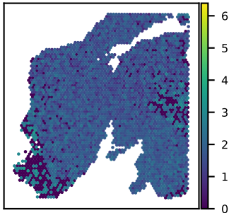
SNU24A PSMD4 expression Moran's I = 0.09
