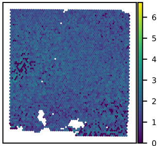
SNU43A TMEM230 expression Moran's I = 0.09
