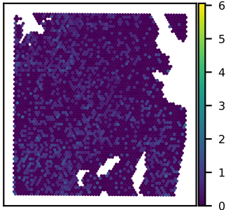
SNU51A ENPEP expression Moran's I = 0.05
