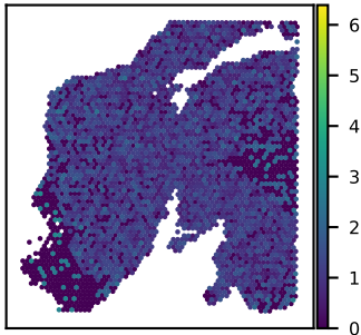
SNU24A RABGAP1 expression Moran's I = 0.08
