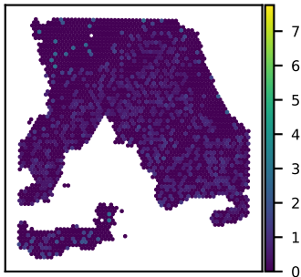
SNU18A NPRL2 expression Moran's I = 0.02
