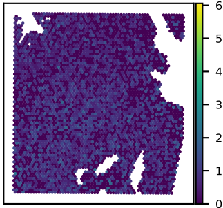
SNU51A TMEM159 expression Moran's I = 0.03
