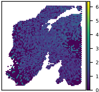
SNU24A CIITA expression Moran's I = 0.16
