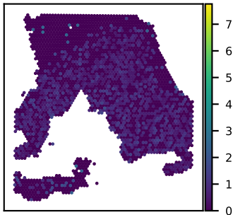
SNU18A SLC9A9 expression Moran's I = 0.09
