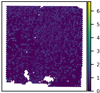
SNU43A CALCRL expression Moran's I = 0.06
