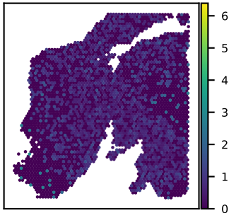
SNU24A TMEM170B expression Moran's I = 0.03
