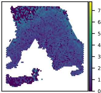
SNU18A RNF213 expression Moran's I = 0.28
