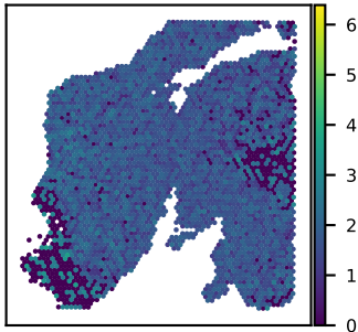
SNU24A MAP4K4 expression Moran's I = 0.14
