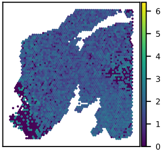
SNU24A SERPINE2 expression Moran's I = 0.15
