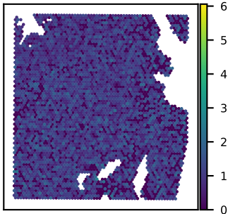
SNU51A RAB11B expression Moran's I = 0.02
