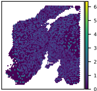
SNU24A NECTIN3 expression Moran's I = 0.03
