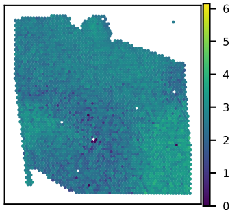
SNU27A IDS expression Moran's I = 0.52
