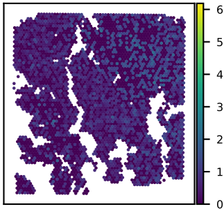
SNU16B PRTFDC1 expression Moran's I = 0.05
