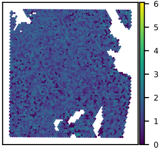
SNU51A RNASEK expression Moran's I = 0.04
