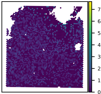
SNU21B YWHAE expression Moran's I = 0.05
