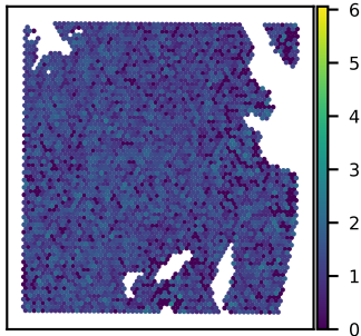
SNU51A SNRPC expression Moran's I = 0.05
