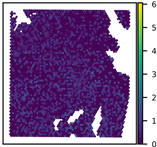
SNU51A DONSON expression Moran's I = 0.03
