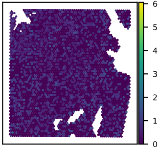
SNU51A AP3B1 expression Moran's I = 0.01
