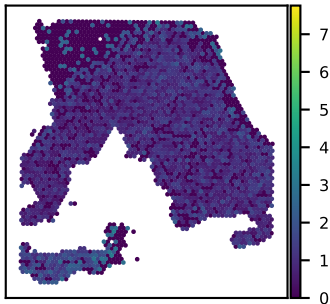
SNU18A PCNX2 expression Moran's I = 0.10
