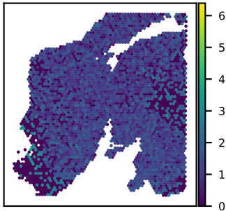
SNU24A PITPNB expression Moran's I = 0.05
