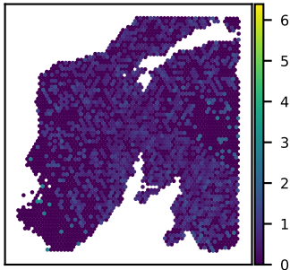
SNU24A SAPCD1 expression Moran's I = 0.06
