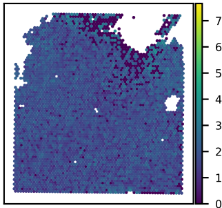
SNU21B TMEM259 expression Moran's I = 0.10
