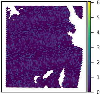
SNU51A CASTOR1 expression Moran's I = 0.01
