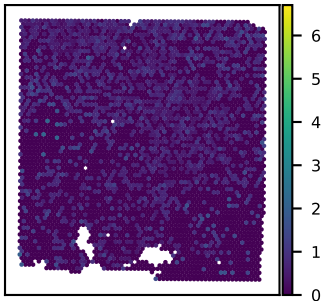
SNU43A C1orf162 expression Moran's I = 0.06
