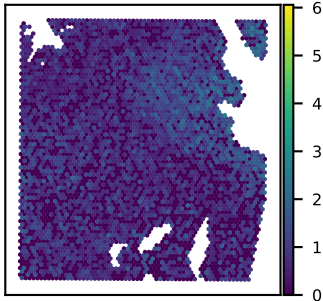
SNU51A MOAP1 expression Moran's I = 0.18
