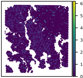
SNU16B CACNG1 expression Moran's I = 0.06
