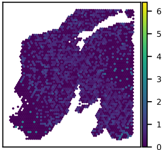
SNU24A C6orf136 expression Moran's I = 0.05
