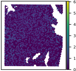
SNU51A ABLIM3 expression Moran's I = 0.03
