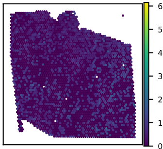
SNU27A LTBP4 expression Moran's I = 0.04
