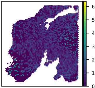
SNU24A ELMOD1 expression Moran's I = 0.05
