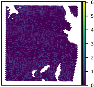
SNU51A RNF122 expression Moran's I = 0.04
