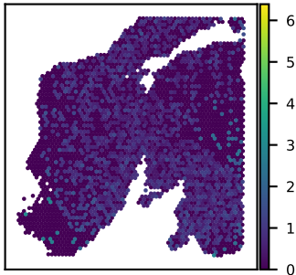
SNU24A CDKN2D expression Moran's I = 0.08
