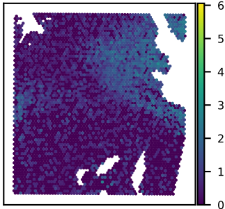
SNU51A NAPB expression Moran's I = 0.50
