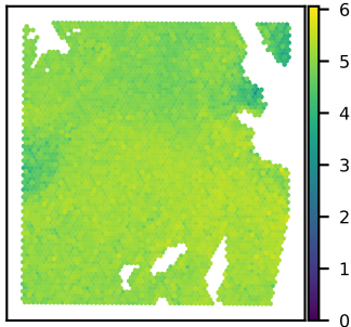
SNU51A CPSF6 expression Moran's I = 0.73
