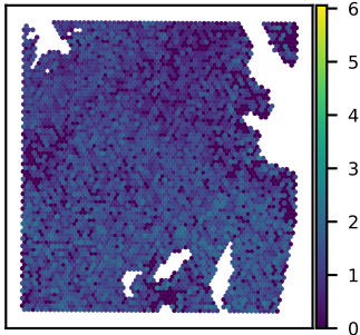
SNU51A DBN1 expression Moran's I = 0.16
